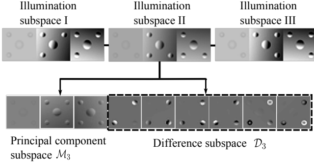
Fig. 6. PCS \mathcal{M}_3 and GDS \mathcal{D}_3 of three 3-dimensional illumination subspaces of different synthetic objects.
