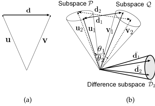
Fig. 2. Conceptual diagram of difference subspace: (a) difference vector \mathbf{d} between \mathbf{u} and \mathbf{v} ; (b) difference subspace \mathcal{D}_2 between N_p -dimensional subspaces \mathcal{P} and N_q -dimensional \mathcal{Q} is defined with the canonical vectors \mathbf{u}_i \in \mathcal{P} and \mathbf{v}_i \in \mathcal{Q} forming the i th canonical angle \theta_i between them. The orthogonal bases \{\tilde{\mathbf{d}}_i\}_{i=1}^{N_p} of \tilde{\mathcal{D}}_2 are obtained by normalizing the difference vectors \mathbf{d}_i between \mathbf{u}_i and \mathbf{v}_i .
