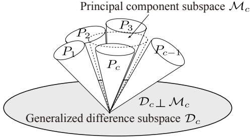
Fig. 5. Conceptual diagram of GDS \mathcal{D}_C for C subspaces \{\mathcal{P}_k\}_{k=1}^C , obtained by removing the PCS \mathcal{M}_C from the sum subspace of the subspaces.
