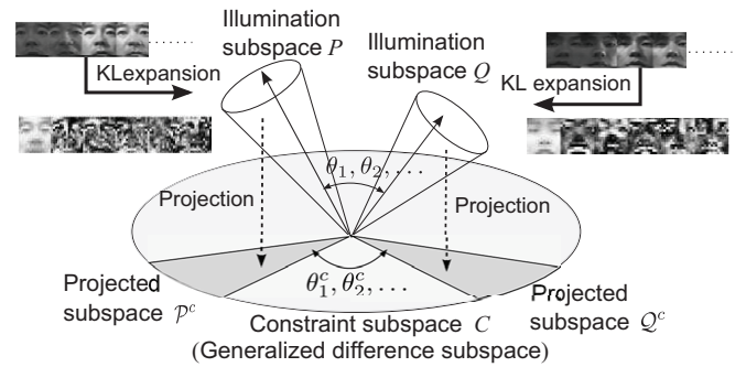
Fig. 1. Conceptual diagram of the constrained mutual subspace method. The canonical angles \{\theta^c\} between the two projected subspaces \mathcal{P}^c and \mathcal{Q}^c onto the GDS are measured. Since it is not possible to depict the subspaces in a high-dimensional space, we show these schematically.
